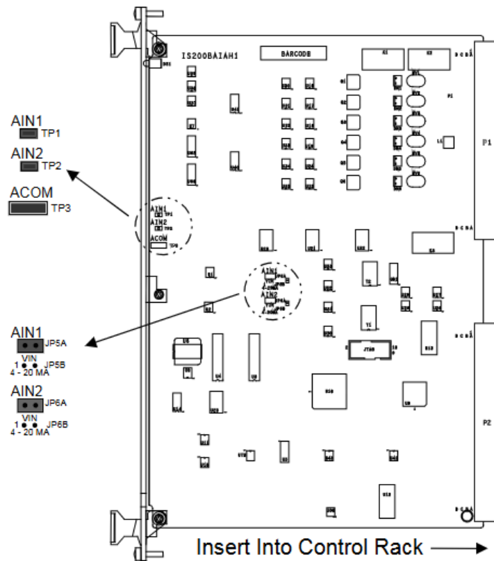
Figure 1 BAIA Board, Side View
