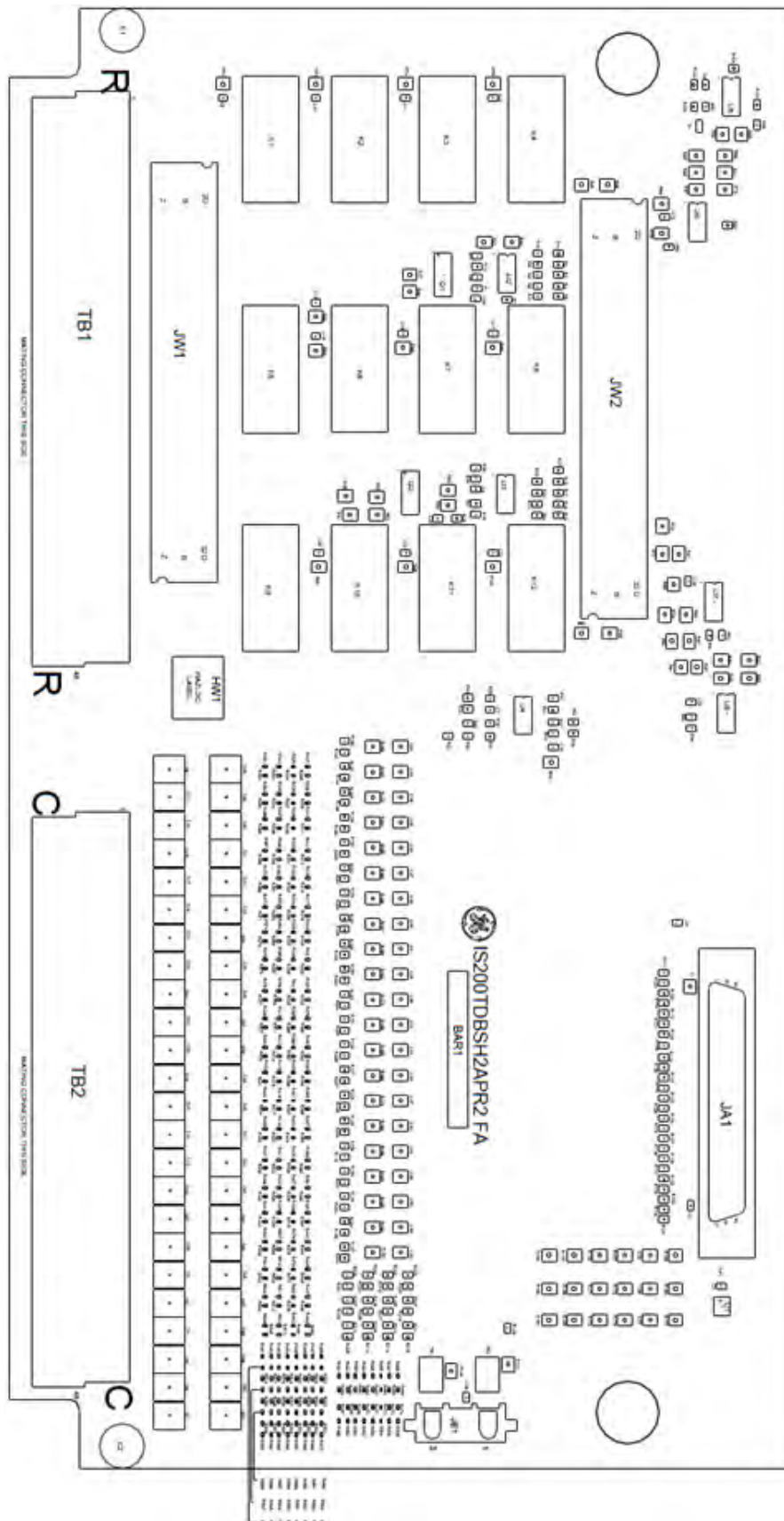
TDBS Layout
