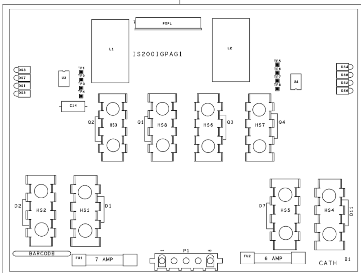
Figure 3. IGPA Board Layout, Group 1
