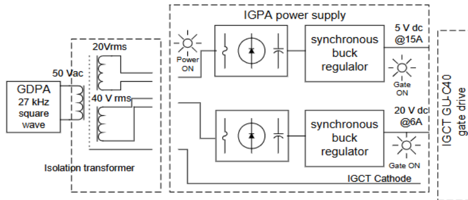
Figure 1. IGPA Functional Diagram
