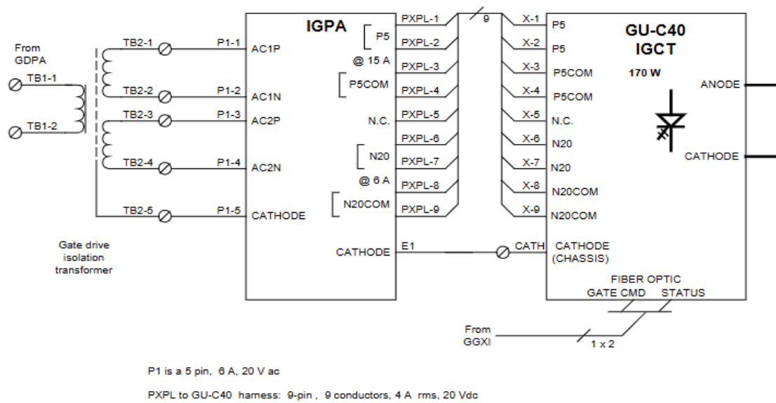
Figure 2. IGPA Connection Diagram
