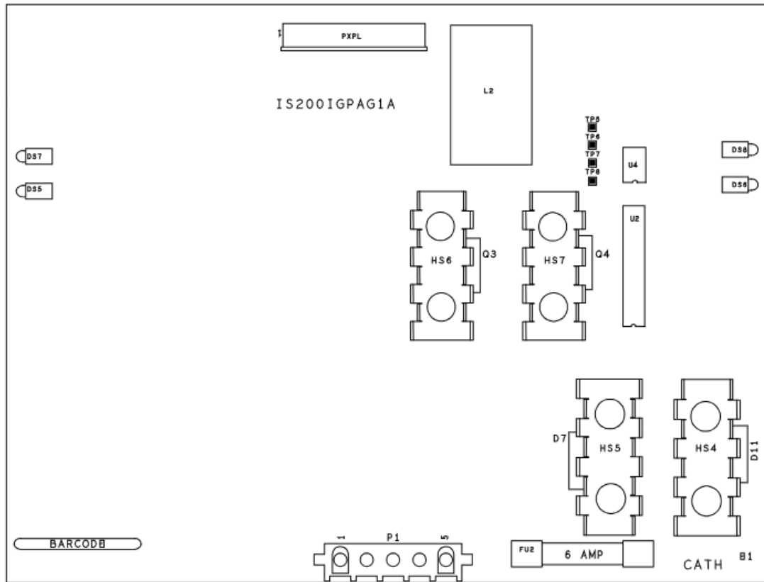
Figure 4. IGPA Board Layout, Group 2
