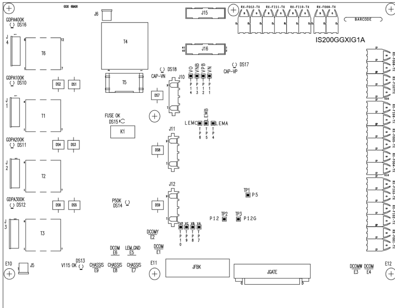
Figure 3. GGXI Board Layout Diagram
