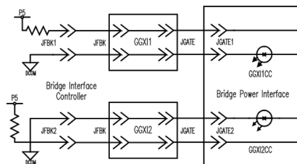
Figure 1. Board Identification Signals
