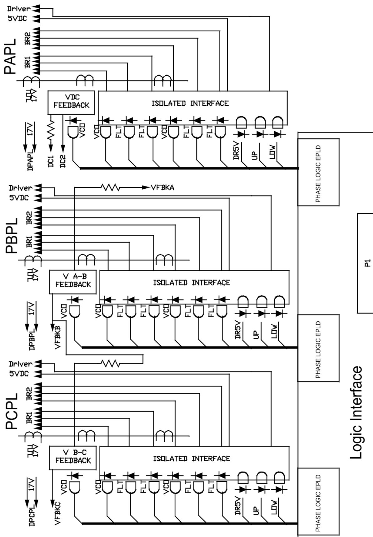
Figure 1. BPIB Board Block Diagram
