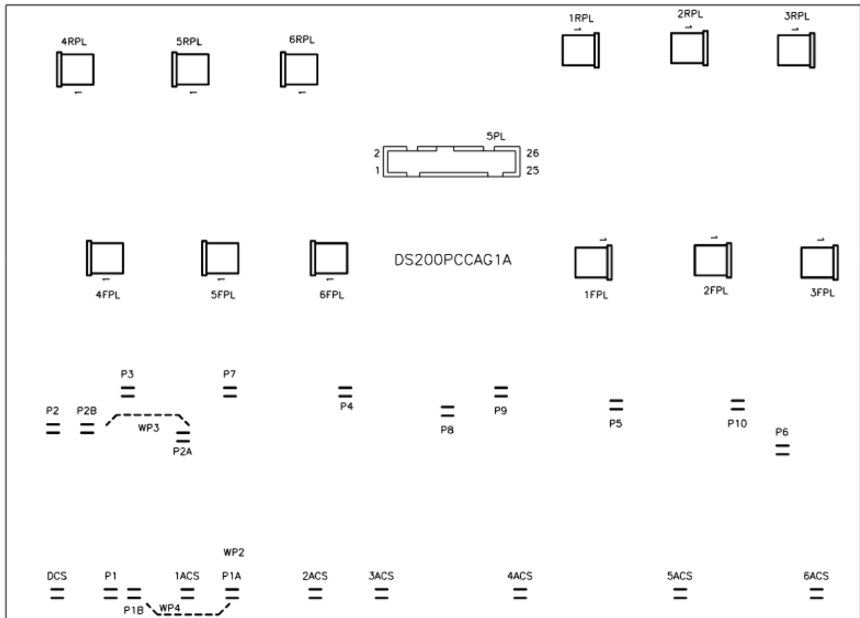
Figure 1. PCCA Card Layout Diagram
